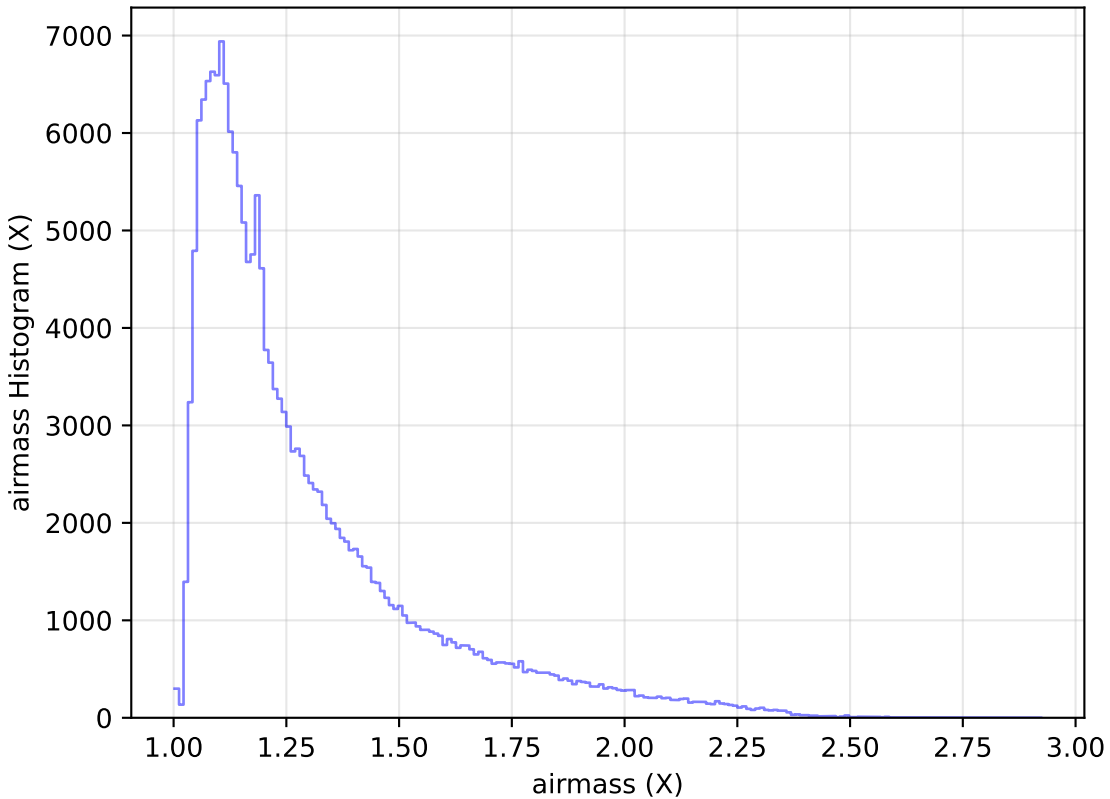
too_elab_r8_d2_ugrizy_v3.4_10yrs All sky g band: airmass Histogram
