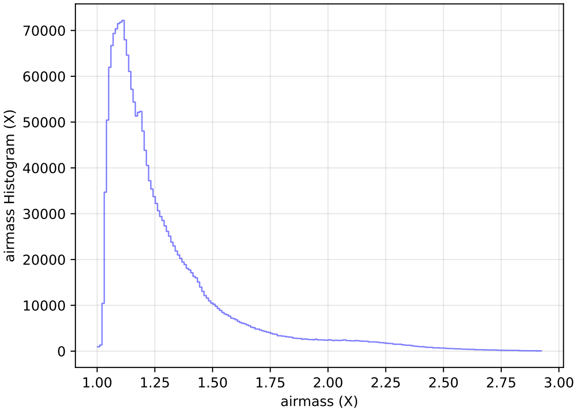
too_elab_r8_d2_ugrizy_v3.4_10yrs All sky all bands: airmass Histogram
