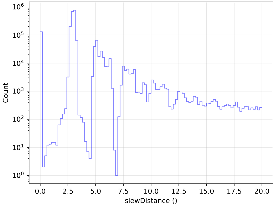
too_elab_r8_d2_ugrizy_v3.4_10yrs All visits: Zoom Slew Distance Histogram
