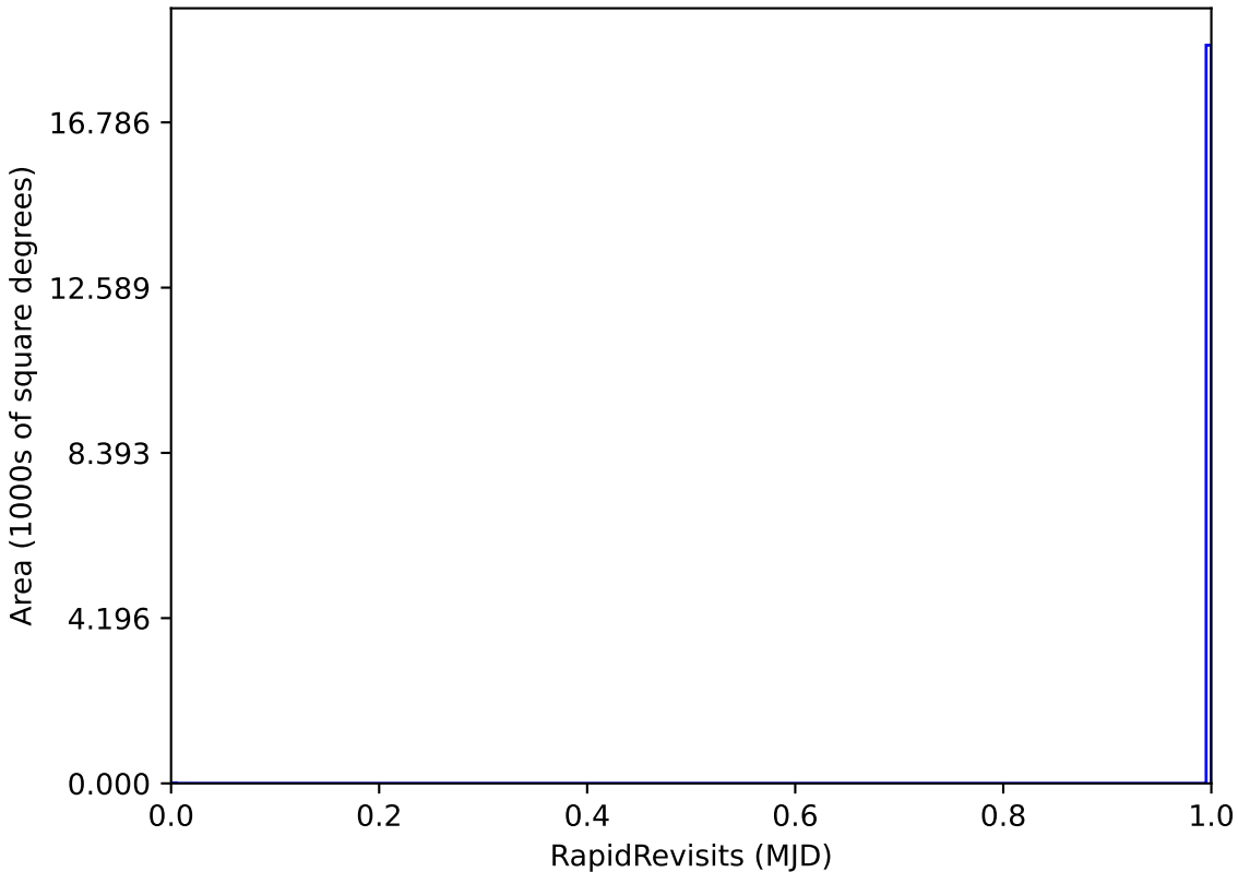
too_elab_r8_d2_ugrizy_v3.4_10yrs WFD: RapidRevisits
