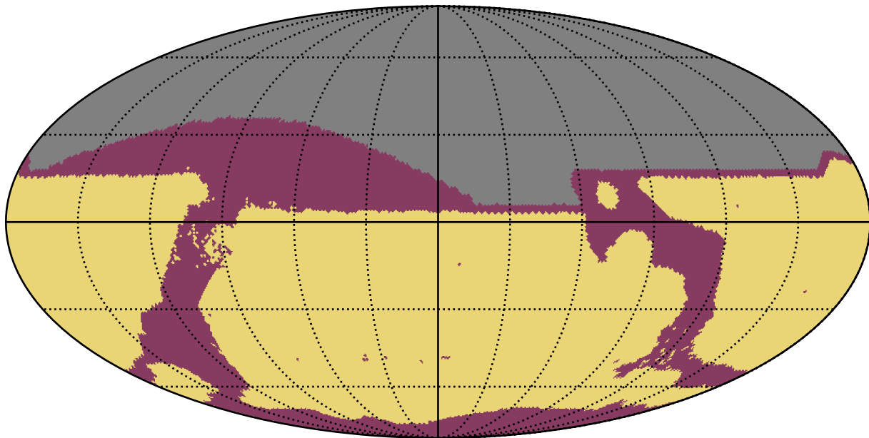
too_elab_r8_d2_ugrizy_v3.4_10yrs All sky: RapidRevisits
