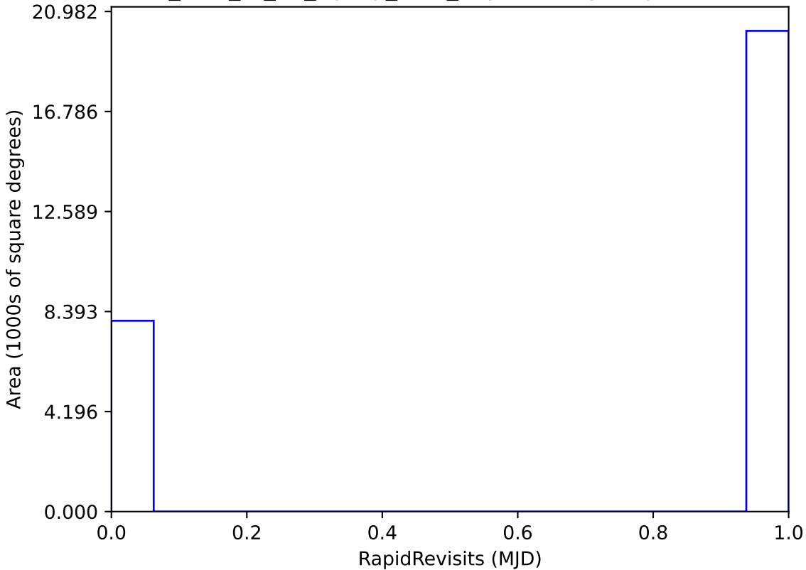
too_elab_r8_d2_ugrizy_v3.4_10yrs All sky: RapidRevisits
