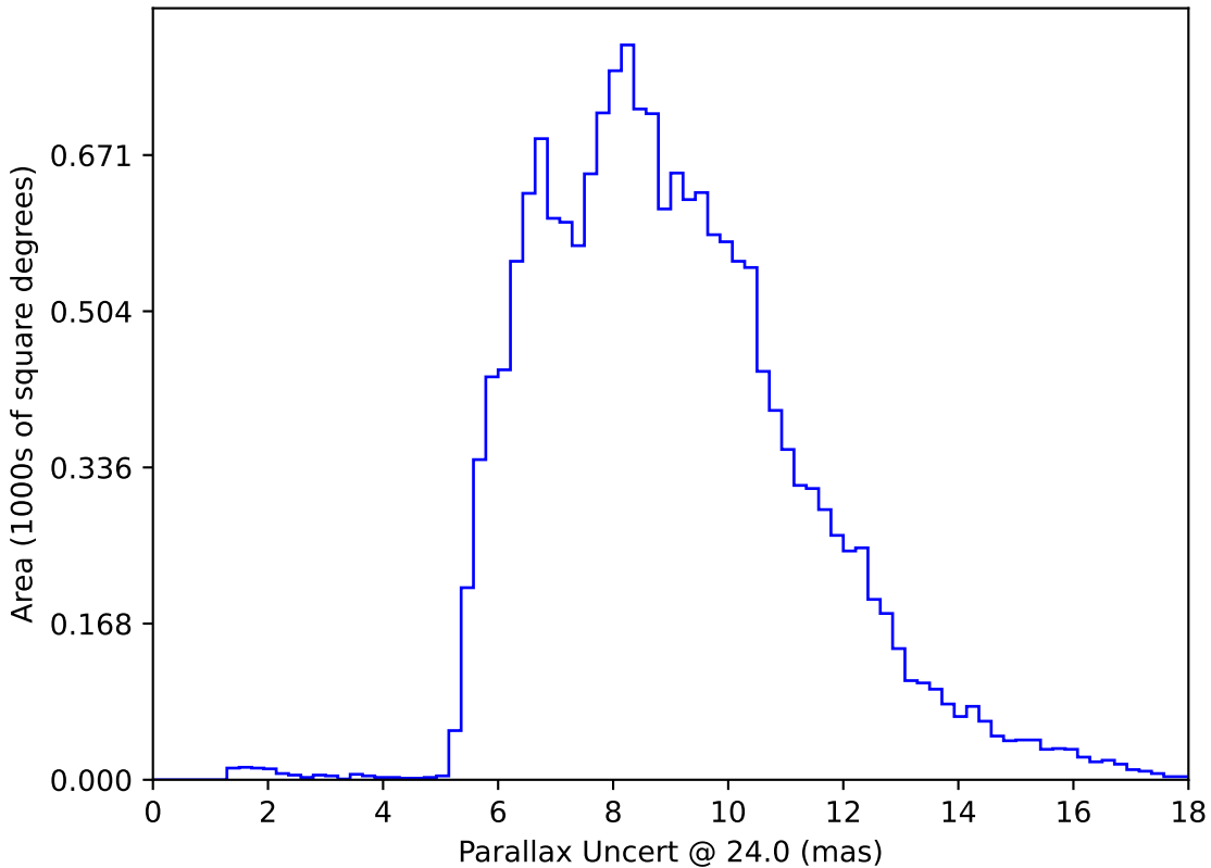
too_elab_r8_d2_ugrizy_v3.4_10yrs WFD: Parallax Uncert @ 24.0
