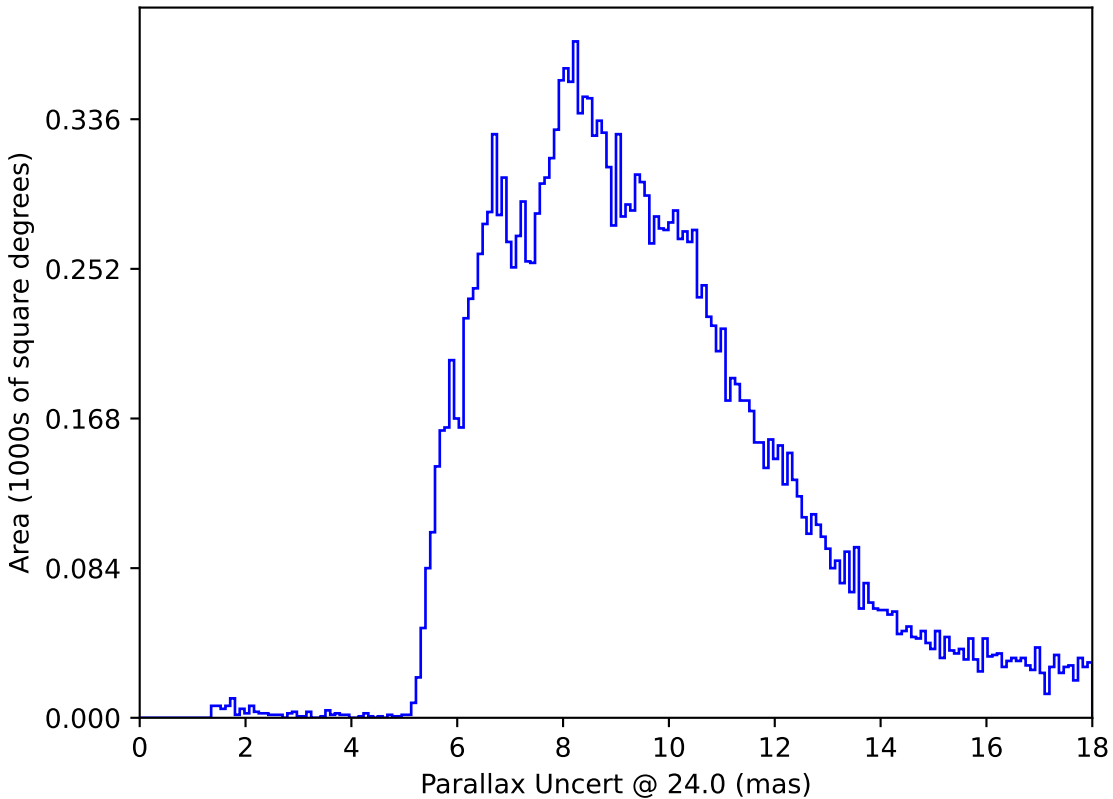
too_elab_r8_d2_ugrizy_v3.4_10yrs All sky: Parallax Uncert @ 24.0
