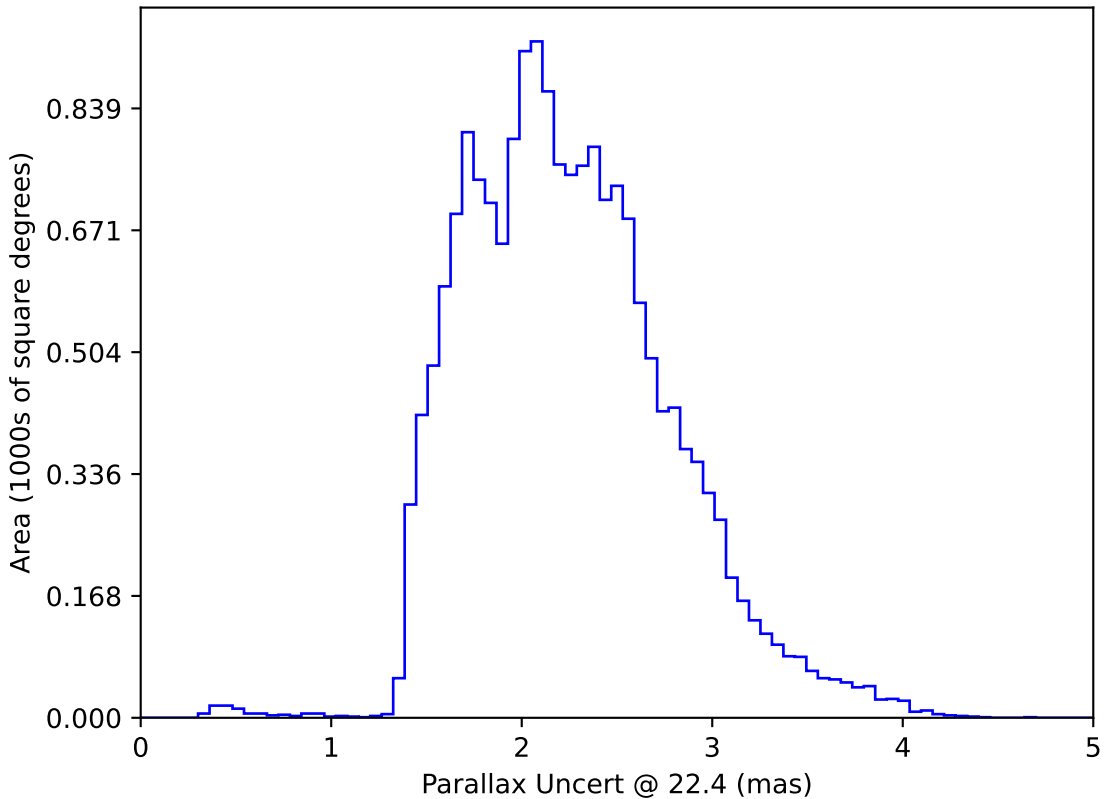
too_elab_r8_d2_ugrizy_v3.4_10yrs WFD: Parallax Uncert @ 22.4
