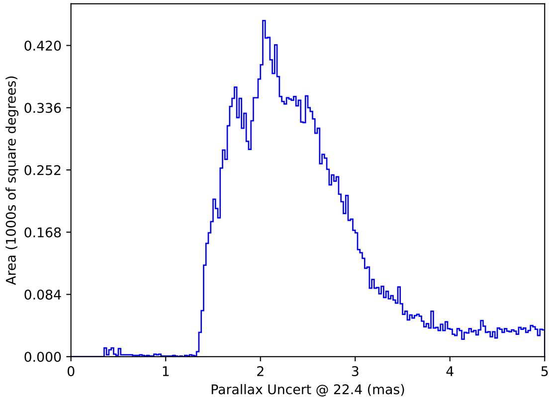
too_elab_r8_d2_ugrizy_v3.4_10yrs All sky: Parallax Uncert @ 22.4
