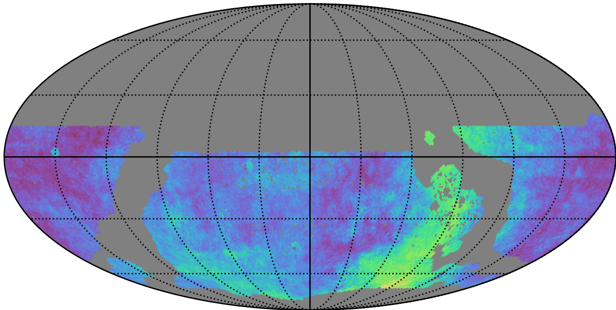
too_elab_r8_d2_ugrizy_v3.4_10yrs WFD: Parallax Coverage @ 24.0
