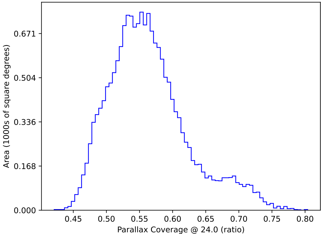
too_elab_r8_d2_ugrizy_v3.4_10yrs WFD: Parallax Coverage @ 24.0
