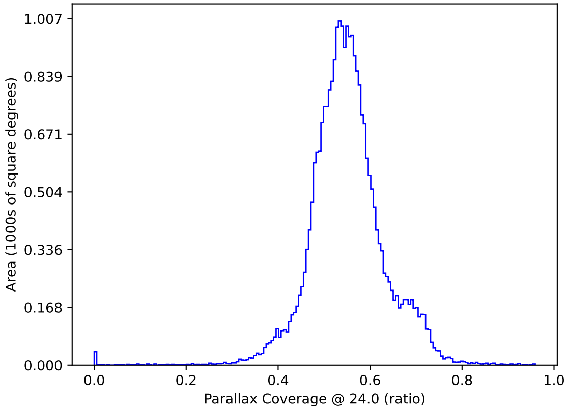
too_elab_r8_d2_ugrizy_v3.4_10yrs All sky: Parallax Coverage @ 24.0
