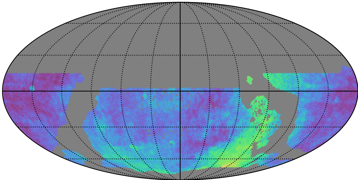
too_elab_r8_d2_ugrizy_v3.4_10yrs WFD: Parallax Coverage @ 22.4
