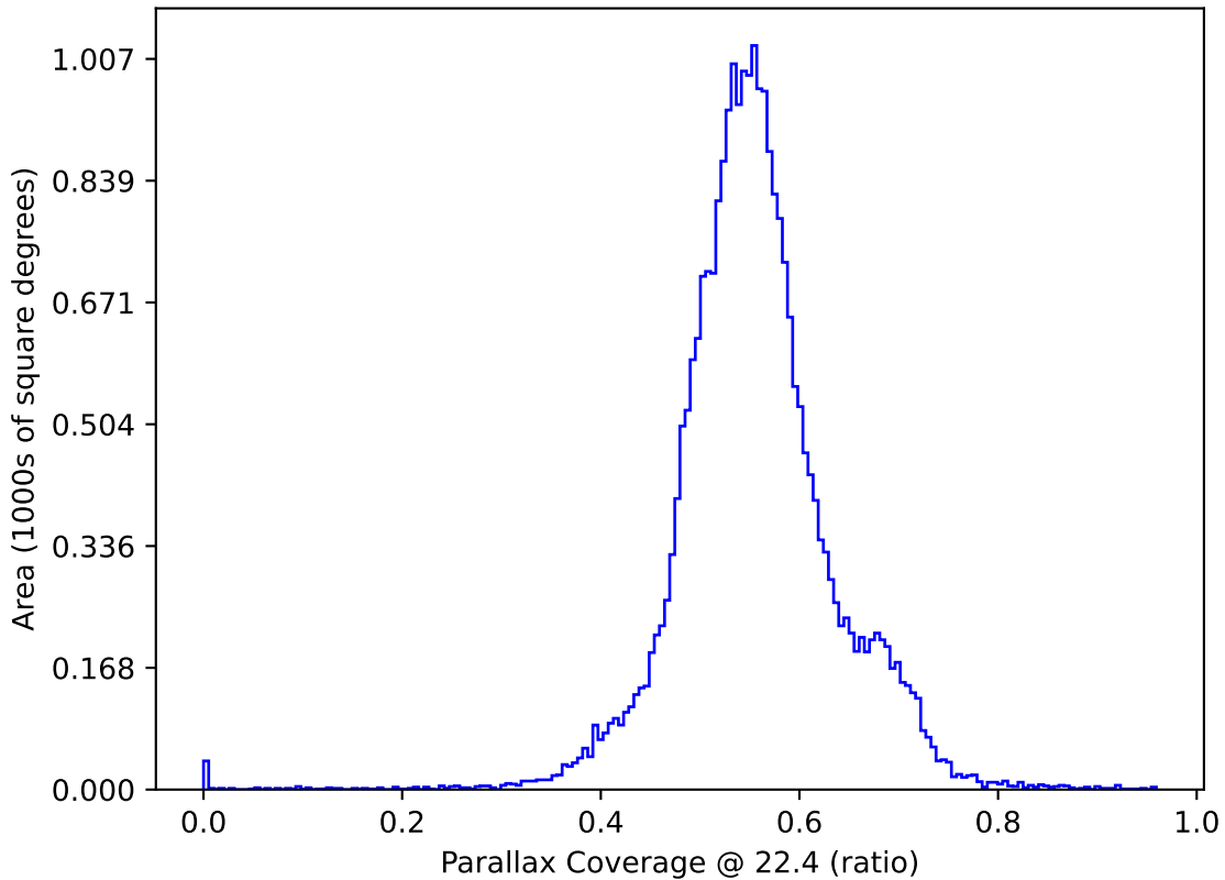
too_elab_r8_d2_ugrizy_v3.4_10yrs All sky: Parallax Coverage @ 22.4
