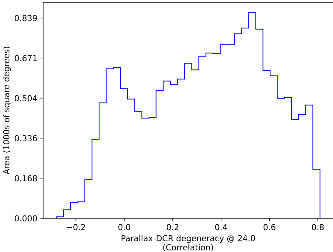
too_elab_r8_d2_ugrizy_v3.4_10yrs WFD: Parallax-DCR degeneracy @ 24.0
