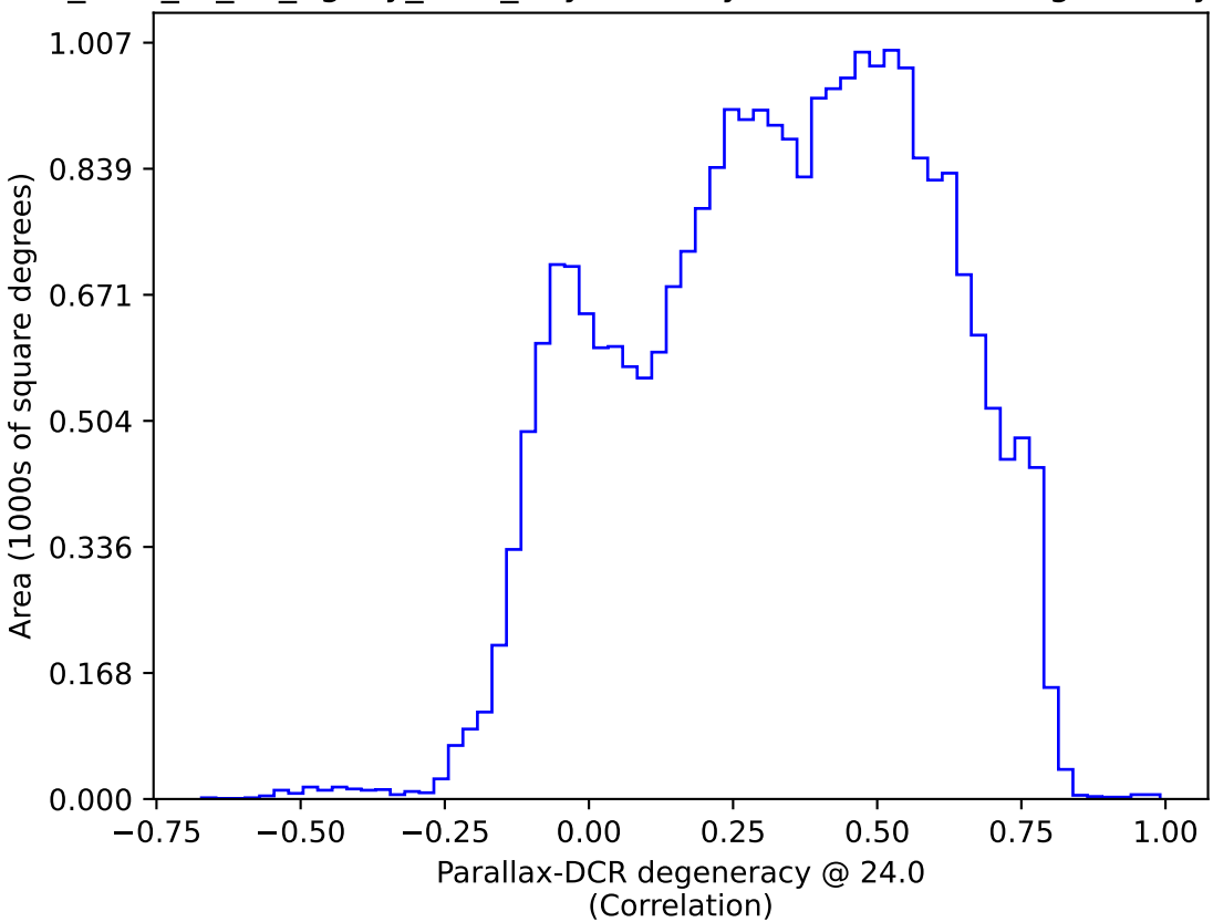
too_elab_r8_d2_ugrizy_v3.4_10yrs All sky: Parallax-DCR degeneracy @ 24.0
