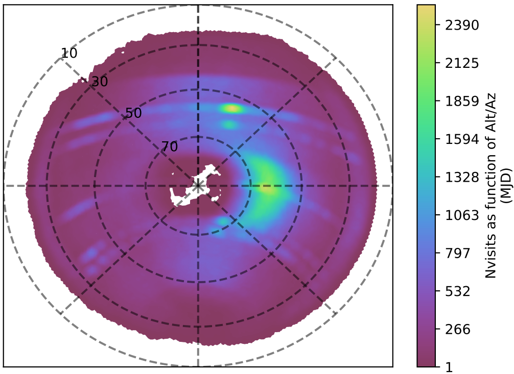
too_elab_r8_d2_ugrizy_v3.4_10yrs z band: Nvisits as function of Alt/Az
