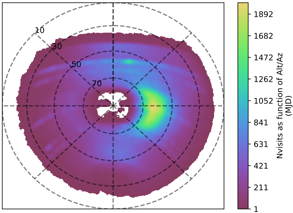
too_elab_r8_d2_ugrizy_v3.4_10yrs y band: Nvisits as function of Alt/Az
