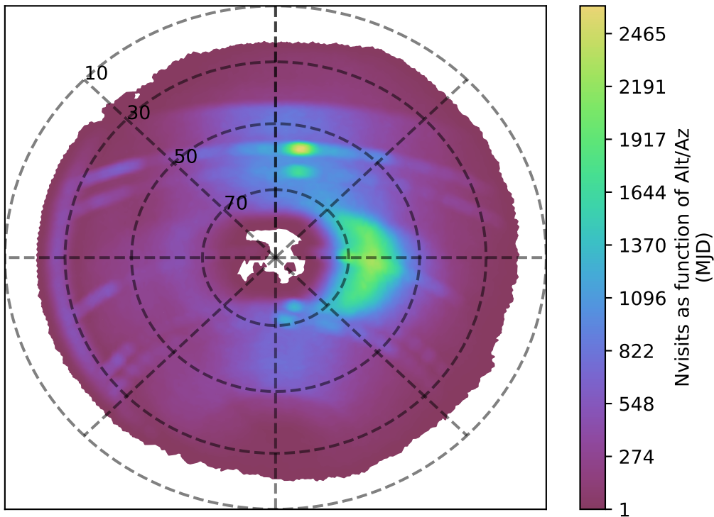
too_elab_r8_d2_ugrizy_v3.4_10yrs r band: Nvisits as function of Alt/Az
