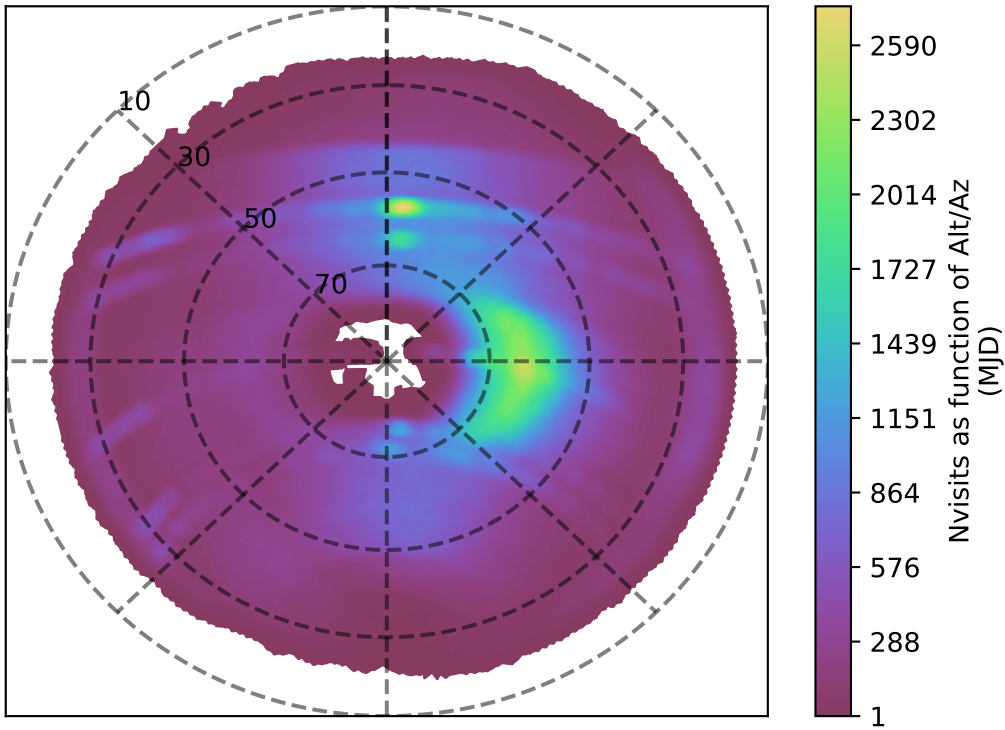
too_elab_r8_d2_ugrizy_v3.4_10yrs i band: Nvisits as function of Alt/Az
