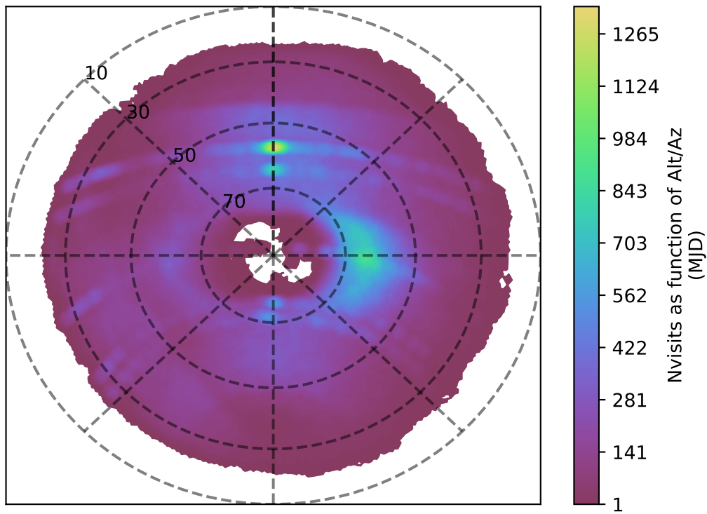
too_elab_r8_d2_ugrizy_v3.4_10yrs g band: Nvisits as function of Alt/Az
