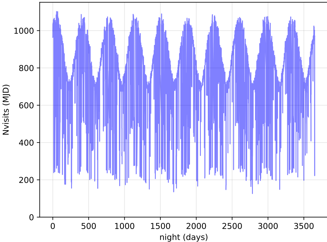
too_elab_r8_d2_ugrizy_v3.4_10yrs All visits: Nvisits
