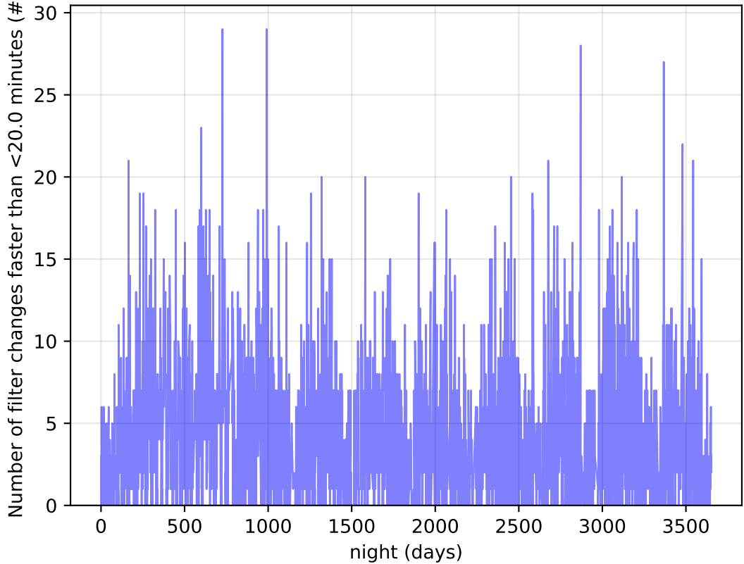
too_elab_r8_d2_ugrizy_v3.4_10yrs Per Night: Number of filter changes faster than <20.0 minutes
