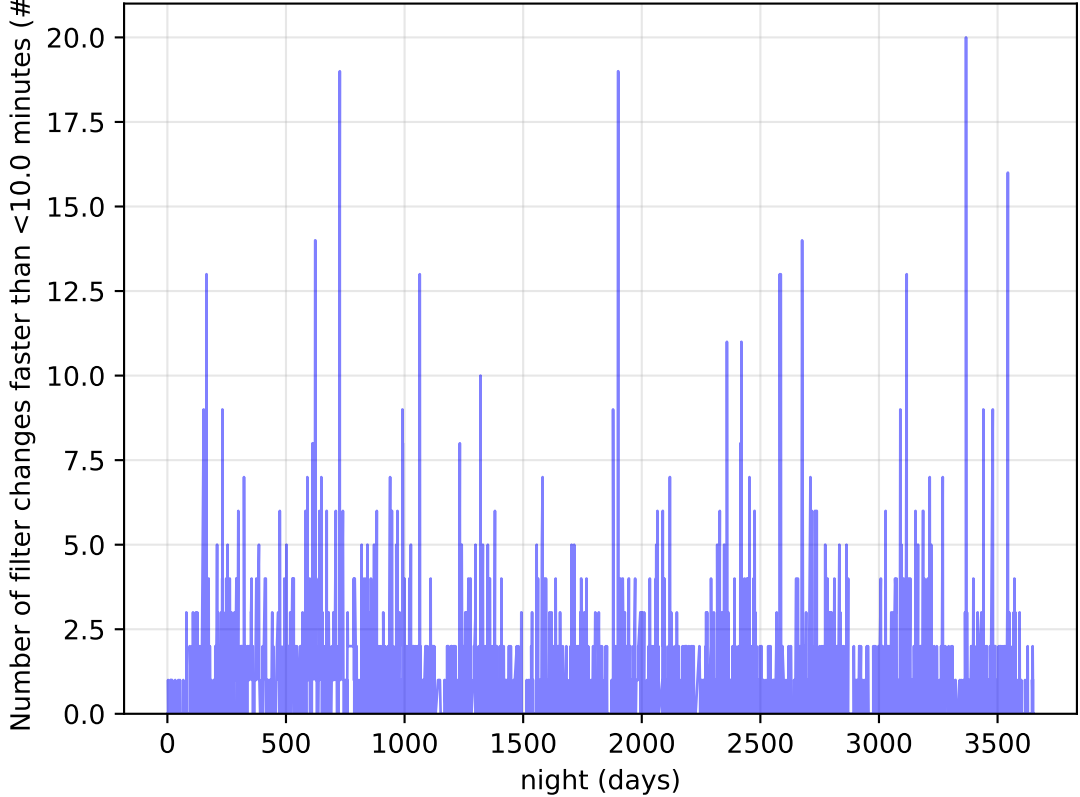
too_elab_r8_d2_ugrizy_v3.4_10yrs Per Night: Number of filter changes faster than <10.0 minutes
