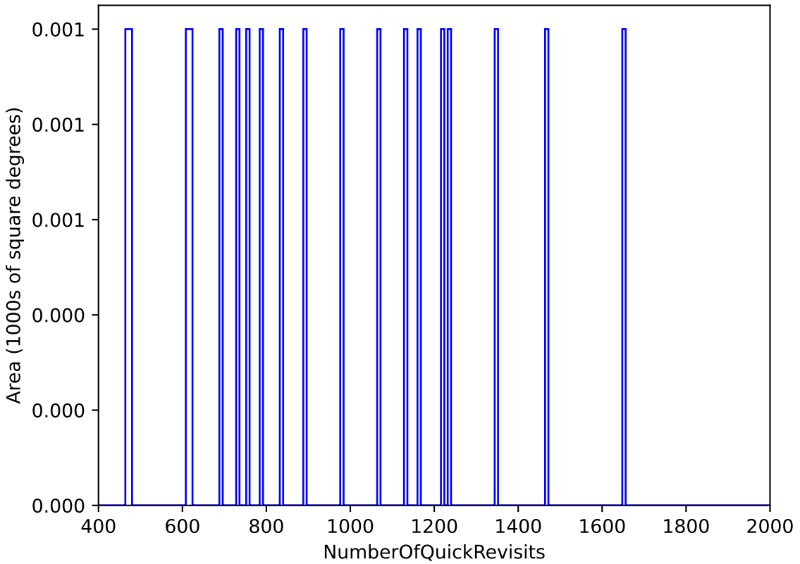
too_elab_r8_d2_ugrizy_v3.4_10yrs WFD: NumberOfQuickRevisits
