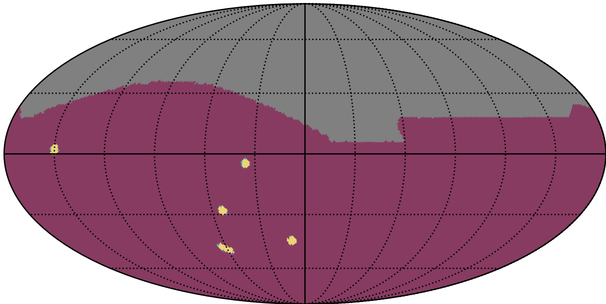
too_elab_r8_d2_ugrizy_v3.4_10yrs All sky: NumberOfQuickRevisits
