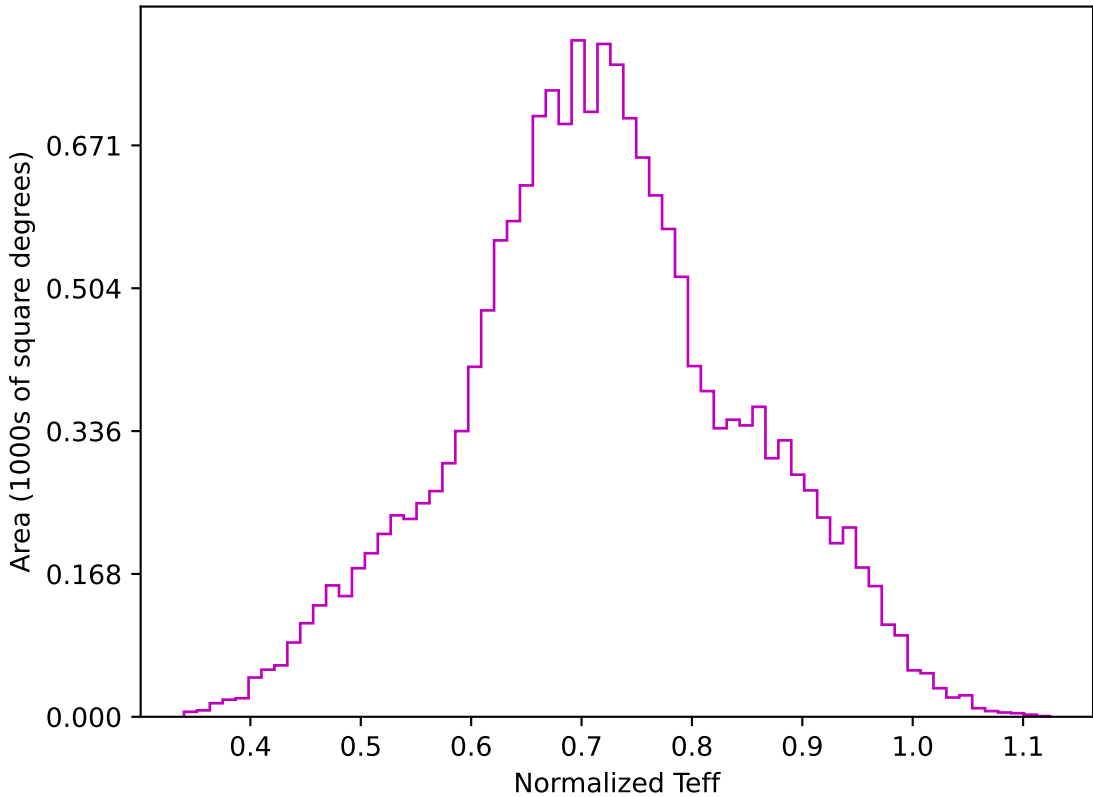
too_elab_r8_d2_ugrizy_v3.4_10yrs WFD z band: Normalized Teff
