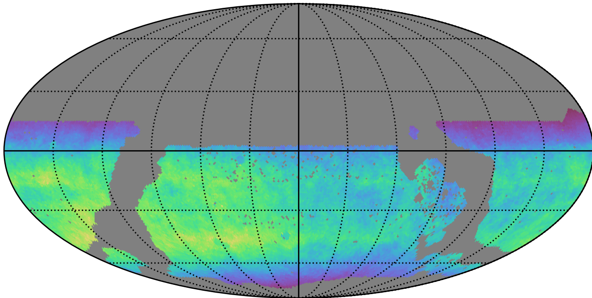
too_elab_r8_d2_ugrizy_v3.4_10yrs WFD y band: Normalized Teff
