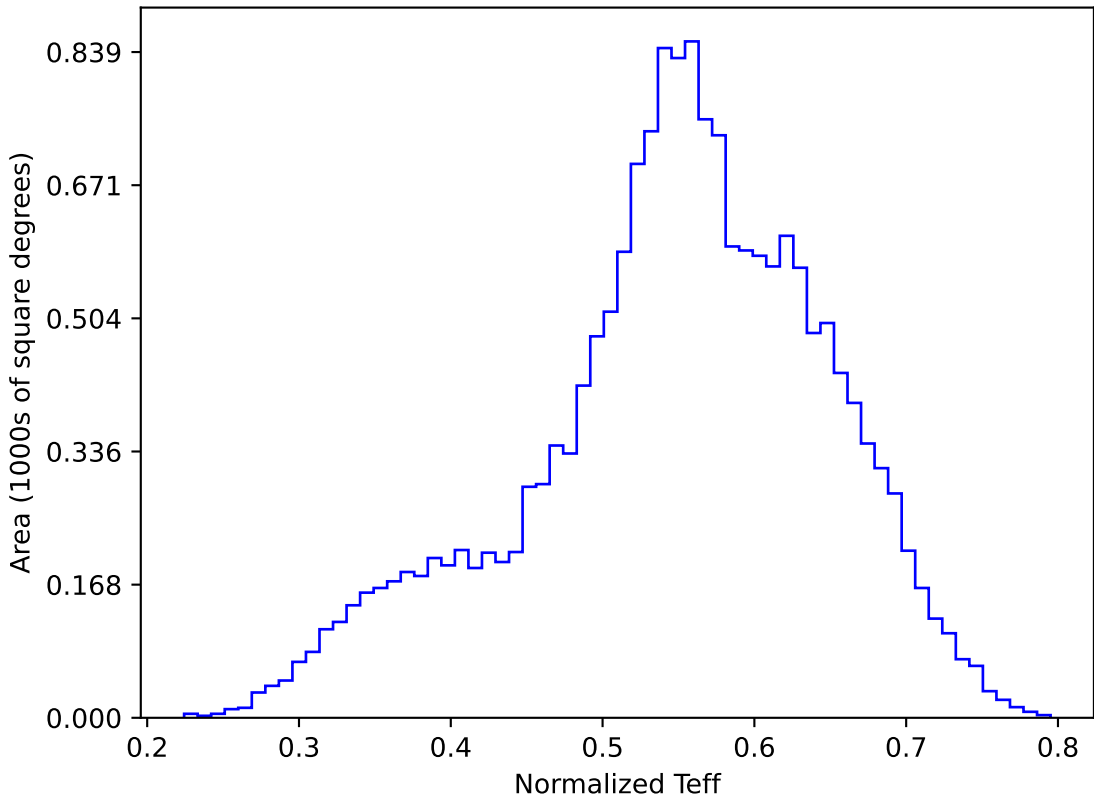
too_elab_r8_d2_ugrizy_v3.4_10yrs WFD y band: Normalized Teff
