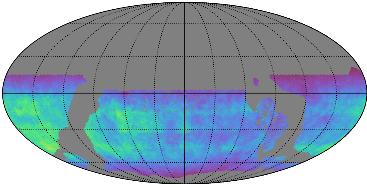
too_elab_r8_d2_ugrizy_v3.4_10yrs WFD u band: Normalized Teff
