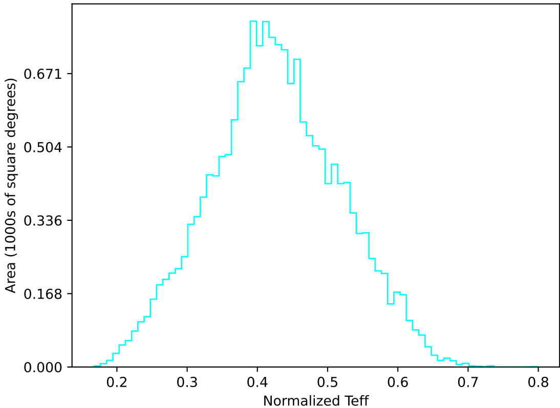
too_elab_r8_d2_ugrizy_v3.4_10yrs WFD u band: Normalized Teff
