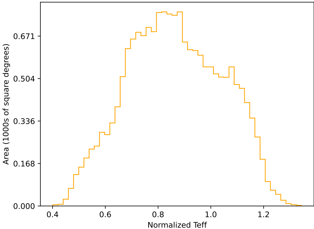
too_elab_r8_d2_ugrizy_v3.4_10yrs WFD r band: Normalized Teff
