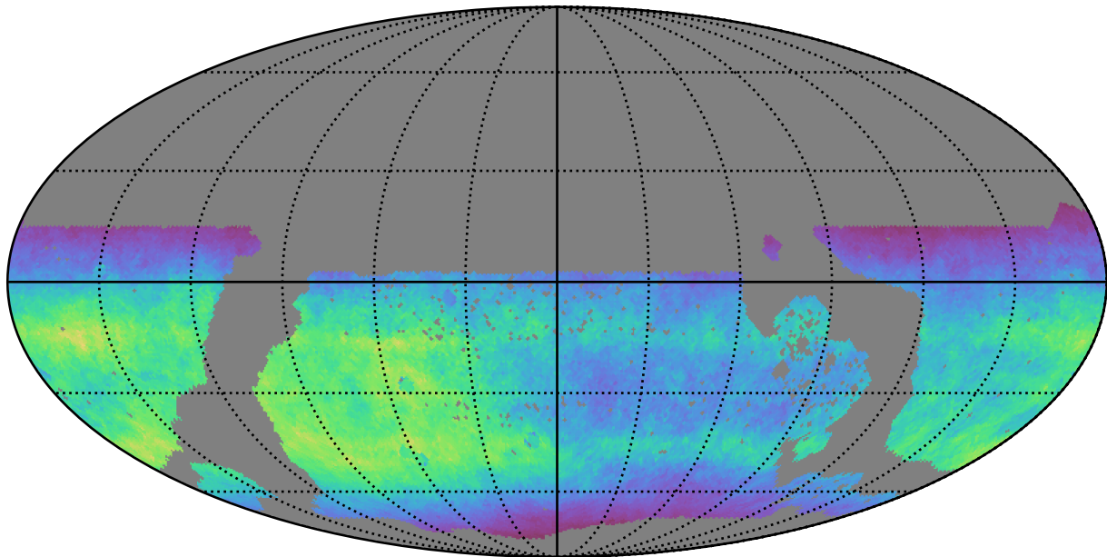
too_elab_r8_d2_ugrizy_v3.4_10yrs WFD i band: Normalized Teff
