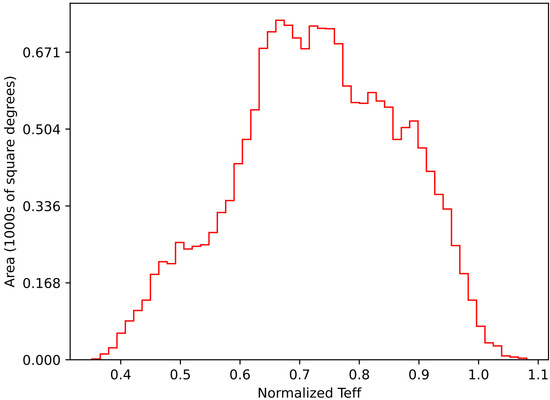
too_elab_r8_d2_ugrizy_v3.4_10yrs WFD i band: Normalized Teff
