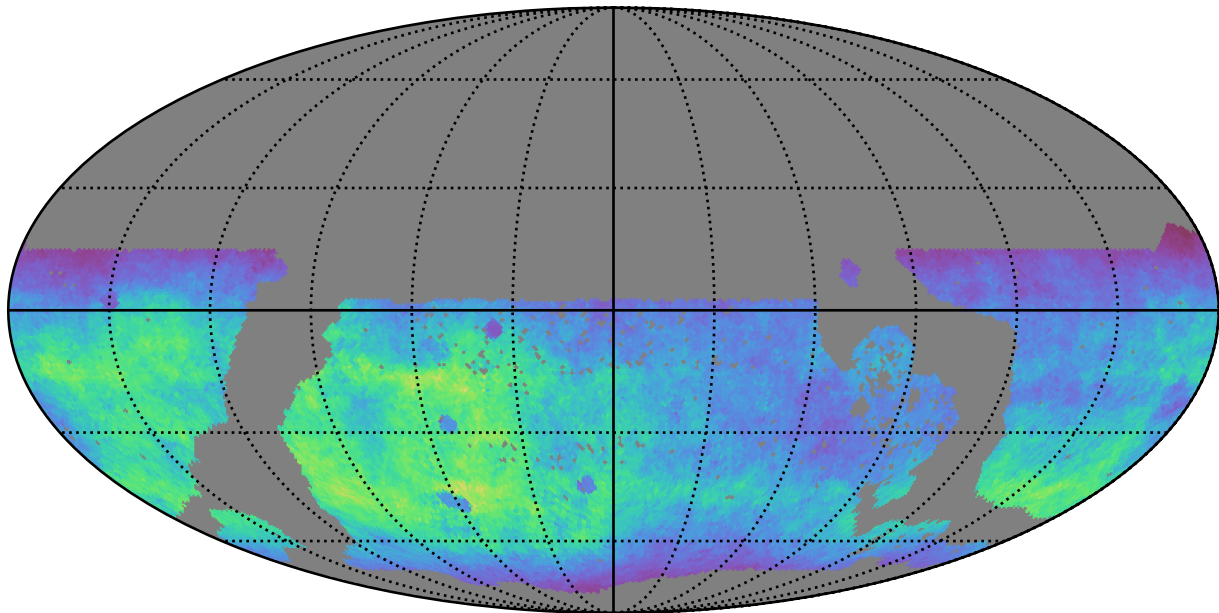
too_elab_r8_d2_ugrizy_v3.4_10yrs WFD g band: Normalized Teff
