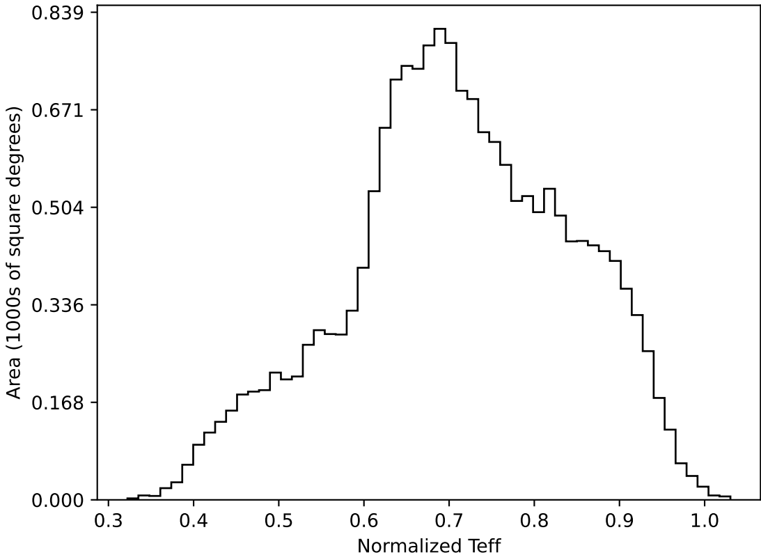
too_elab_r8_d2_ugrizy_v3.4_10yrs WFD all bands: Normalized Teff
