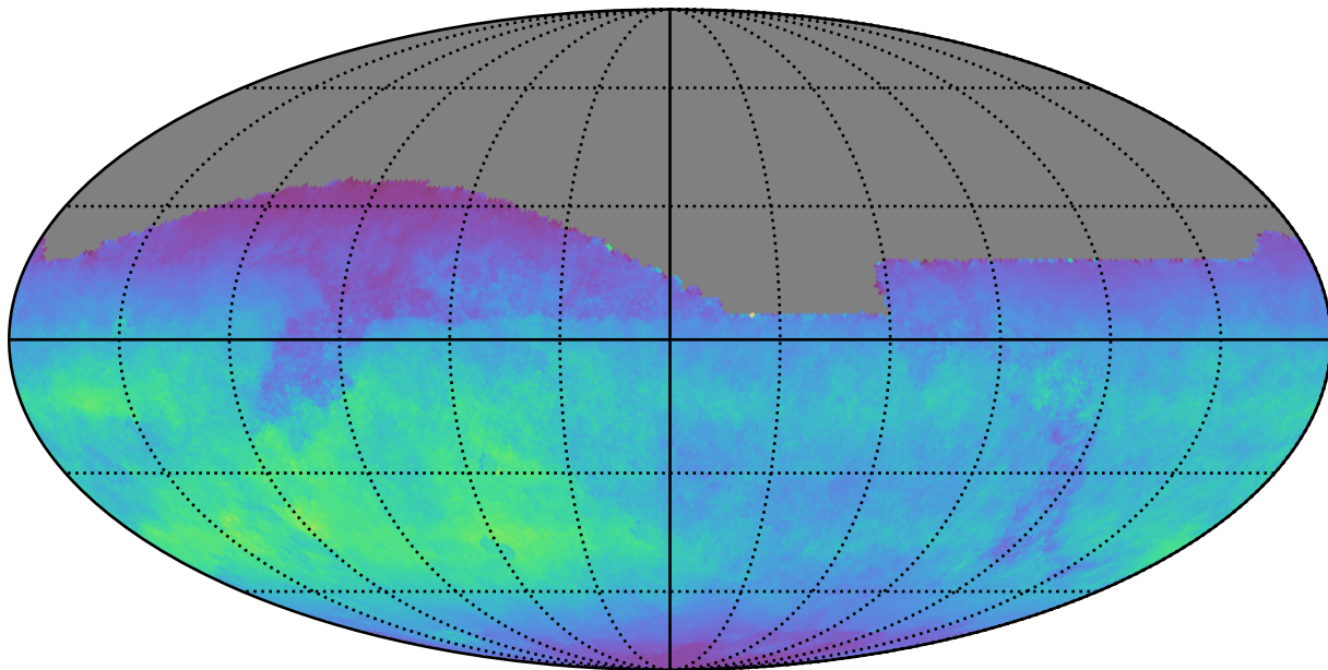
too_elab_r8_d2_ugrizy_v3.4_10yrs All sky z band: Normalized Teff
