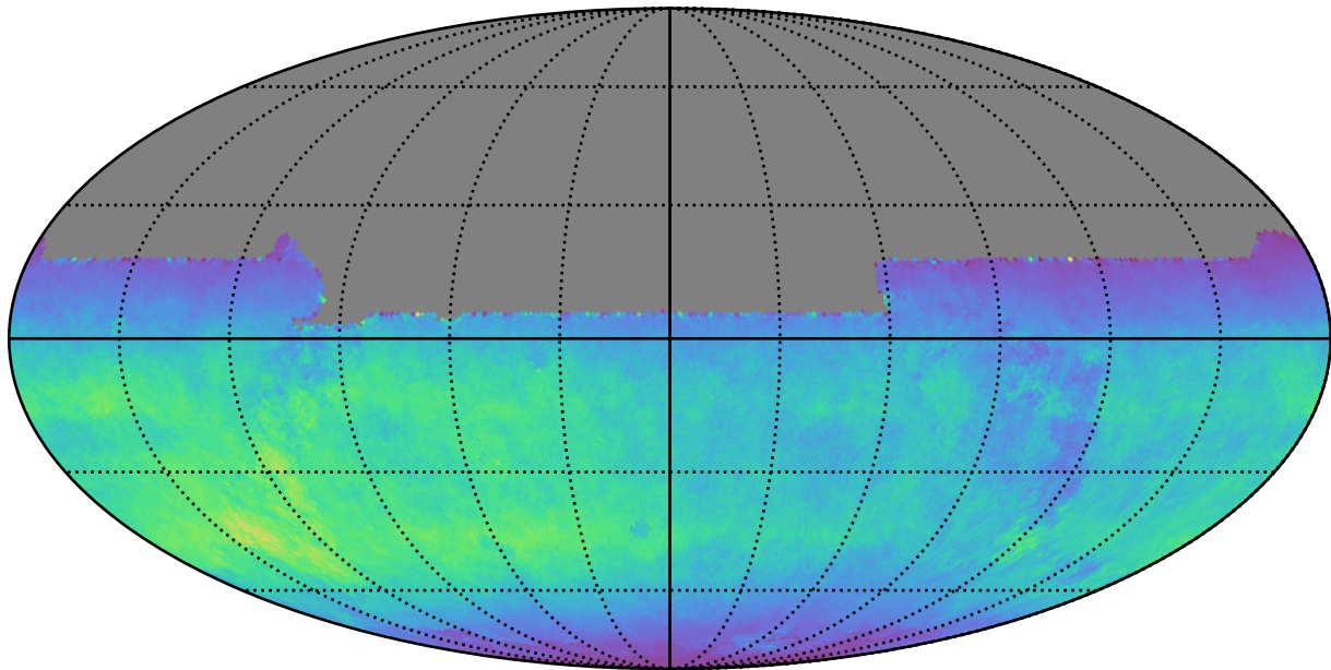
too_elab_r8_d2_ugrizy_v3.4_10yrs All sky y band: Normalized Teff
