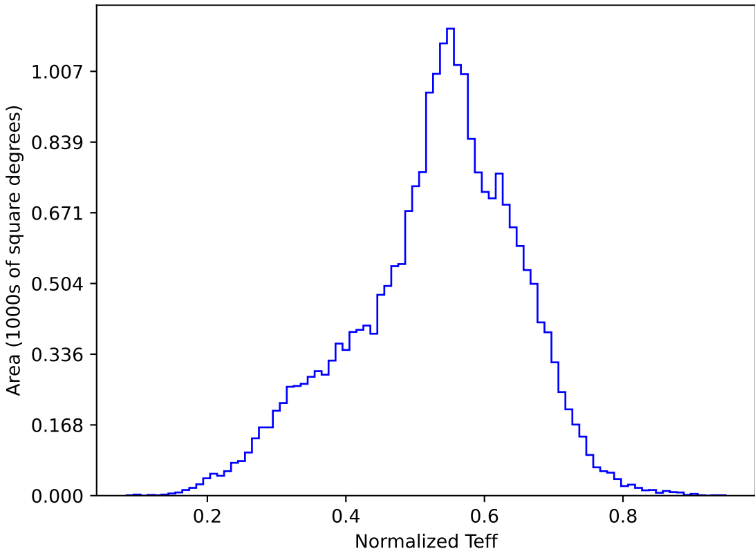
too_elab_r8_d2_ugrizy_v3.4_10yrs All sky y band: Normalized Teff
