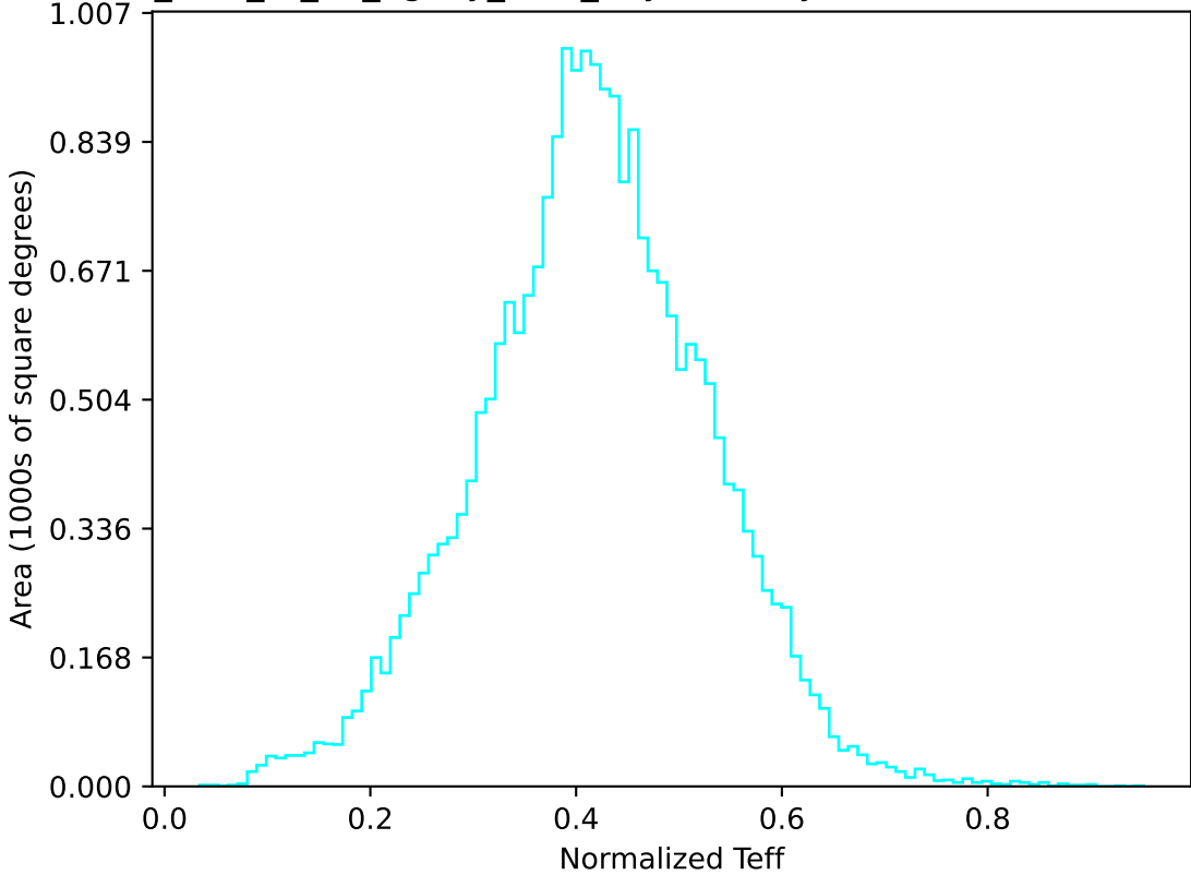
too_elab_r8_d2_ugrizy_v3.4_10yrs All sky u band: Normalized Teff
