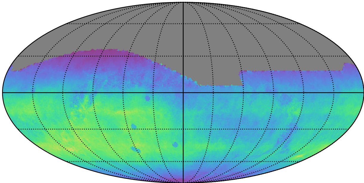
too_elab_r8_d2_ugrizy_v3.4_10yrs All sky r band: Normalized Teff
