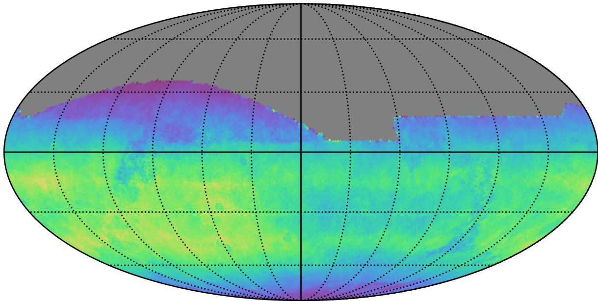
too_elab_r8_d2_ugrizy_v3.4_10yrs All sky i band: Normalized Teff
