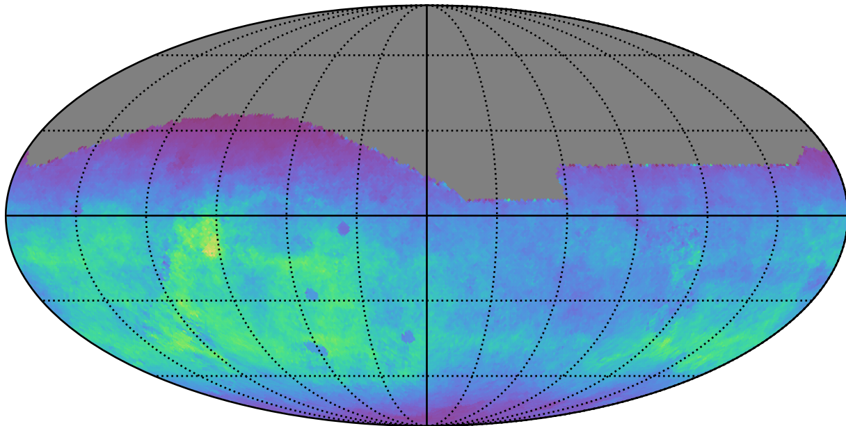
too_elab_r8_d2_ugrizy_v3.4_10yrs All sky g band: Normalized Teff
