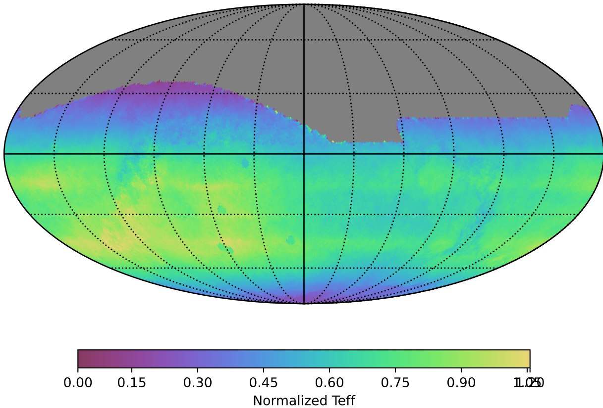
too_elab_r8_d2_ugrizy_v3.4_10yrs All sky all bands: Normalized Teff
