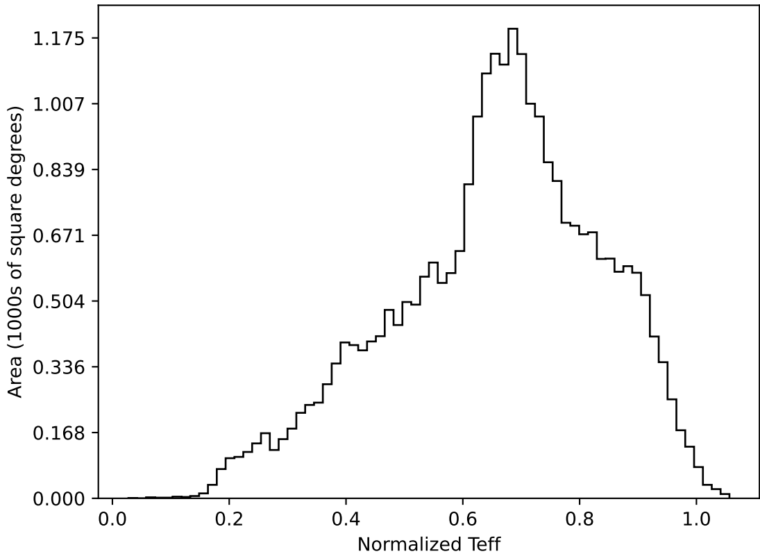
too_elab_r8_d2_ugrizy_v3.4_10yrs All sky all bands: Normalized Teff
