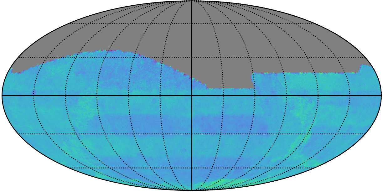
too_elab_r8_d2_ugrizy_v3.4_10yrs All sky: Normalized Proper Motion Uncert @ 24.0
