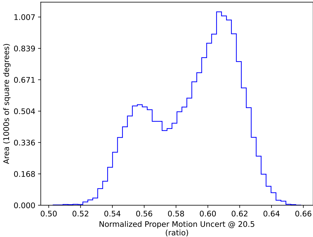
too_elab_r8_d2_ugrizy_v3.4_10yrs WFD: Normalized Proper Motion Uncert @ 20.5
