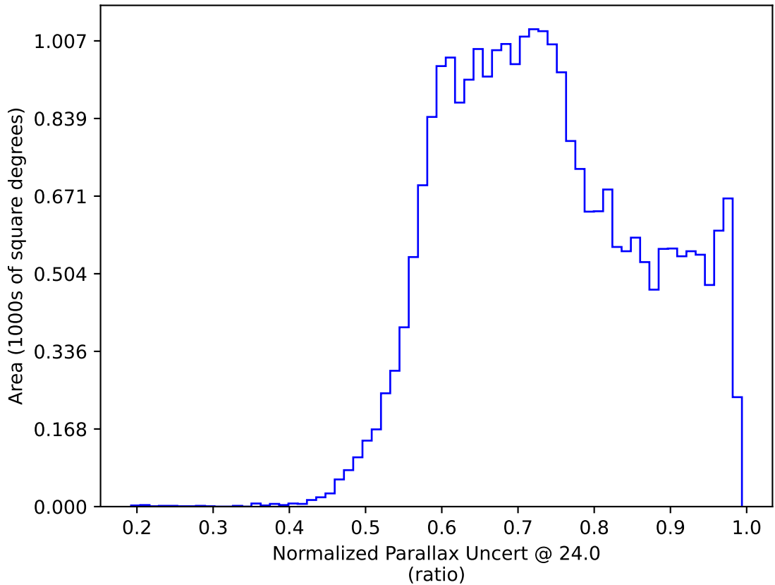
too_elab_r8_d2_ugrizy_v3.4_10yrs All sky: Normalized Parallax Uncert @ 24.0
