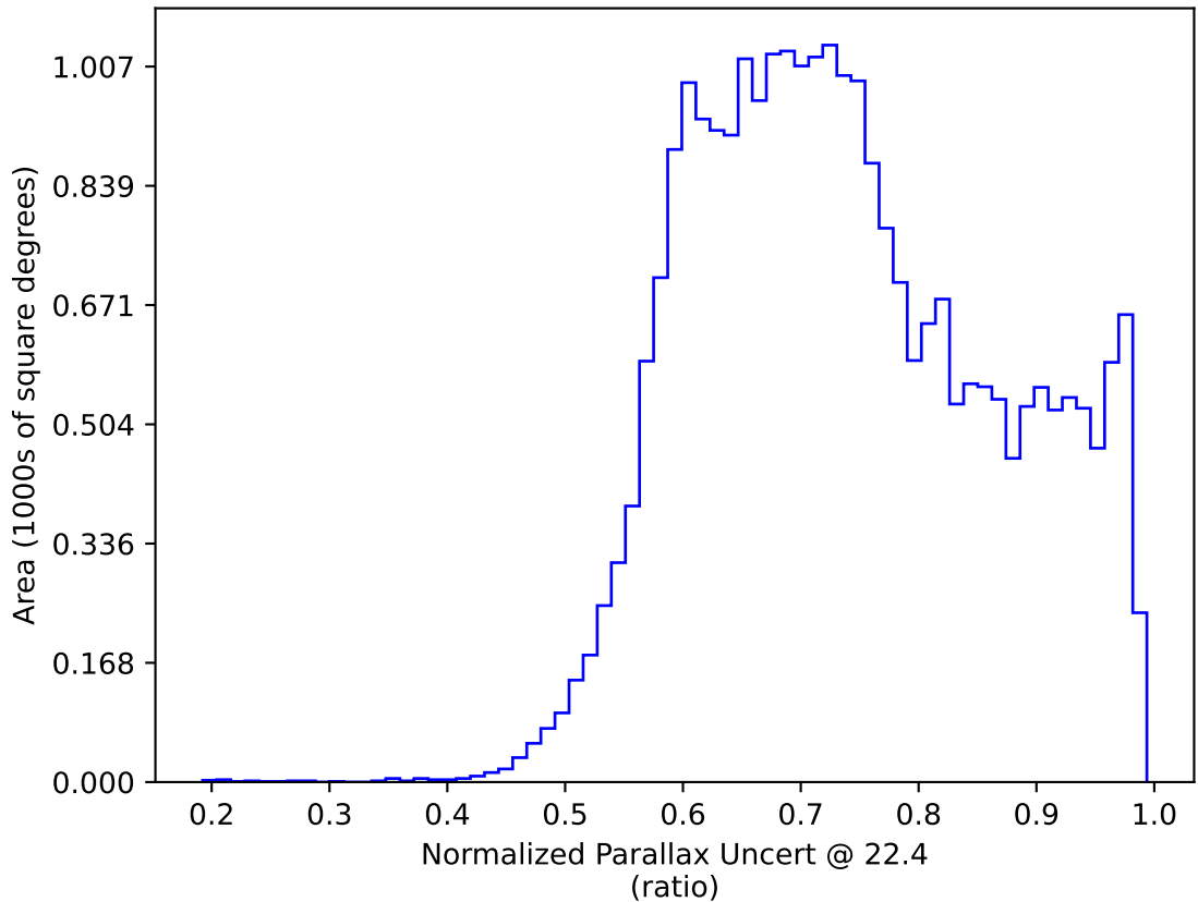
too_elab_r8_d2_ugrizy_v3.4_10yrs All sky: Normalized Parallax Uncert @ 22.4
